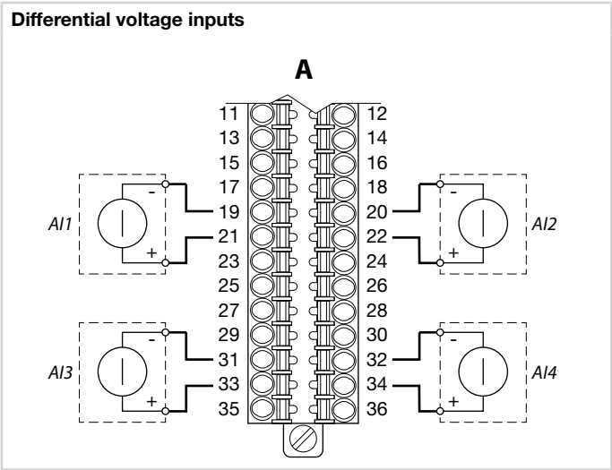
High impedance voltage input
